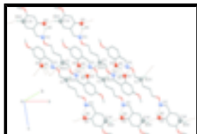
Fig. 2. Part of the supramolecular structure of the title compound. Intra- and intermolecular hydrogen bonds are shown as dashed lines.
